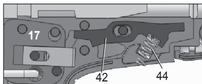
Figure 10: Location of the Trigger Adapter, Sear, and Sear Spring
